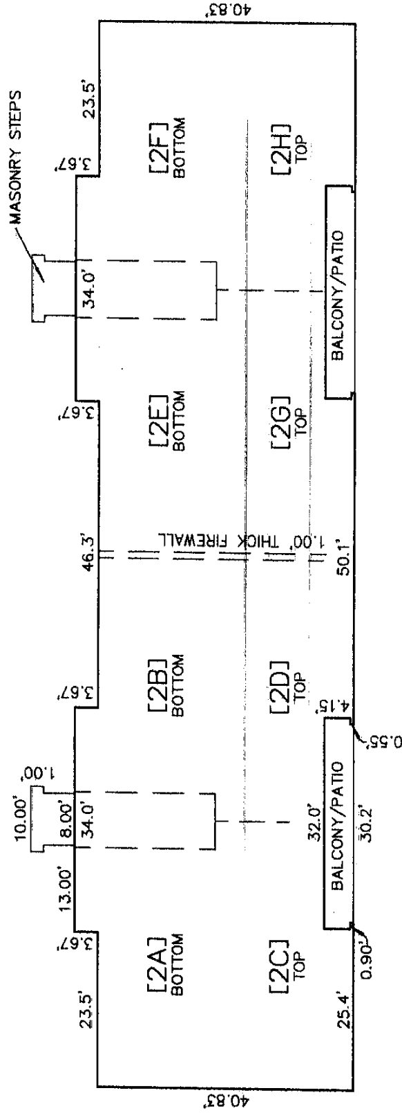
BUILDING NO. 2 FLOORPLAN 3 BEDROOM UNITS
